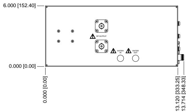
Rear (Output) View
